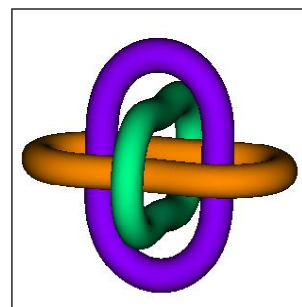
Figure 12. Three dimensional representation of the Borromean link.
