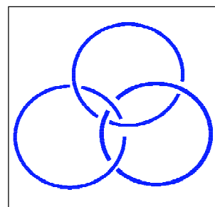
Figure 11. Two dimensional representation of Borromean rings.
