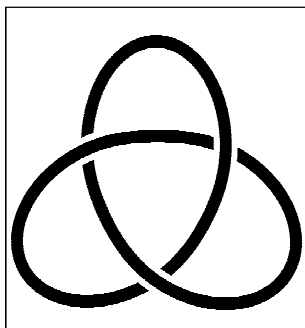
Figure 5. Two dimensional representation of the trefoil. Note that at each intersection, the lower strand is represented by a line that is broken.
