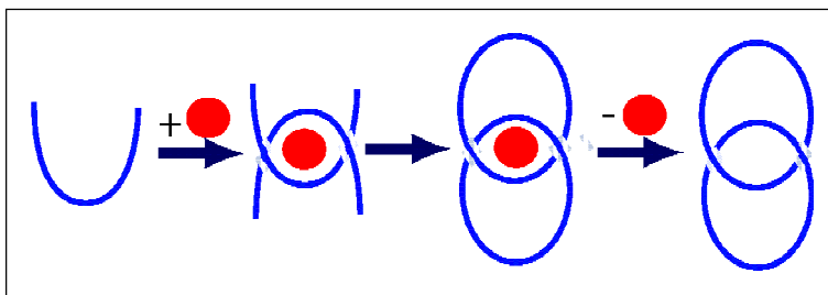
Figure 13. Templated synthesis of [2]catenane.
