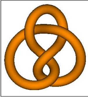
Figure 8. The figure eight knot, which can be represented only with a minimum of four crossings and is labeled as 4_1 .
