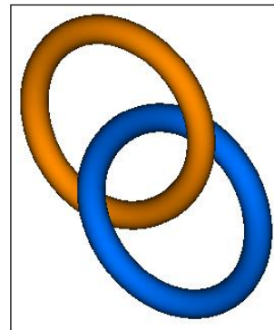
Figure 10. A Hopf link.
