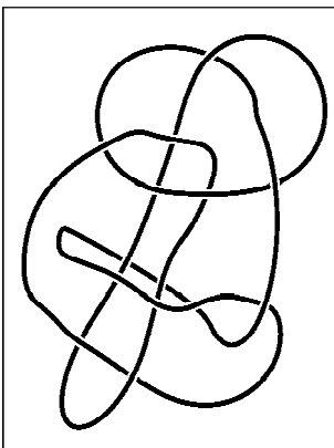
Figure 9. A knot having the same Alexander Polynomial as the unknot. Both have Alexander polynomial equal to unity.
